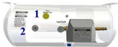
1-Propane fill valve; 2-Propane gauge ASME tank
