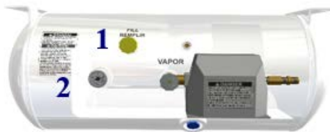
1-Propane fill valve; 2-Propane gauge ASME tank
