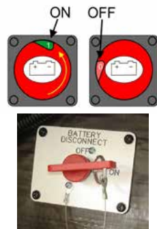
Battery Disconnect Switches (switch appearance may vary by model)
