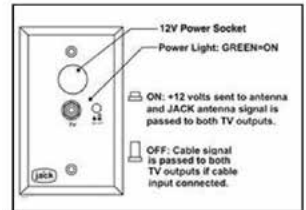
Power Injector
