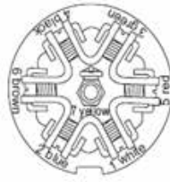
7-way trailer plug-rear view
