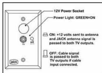
Power Injector
