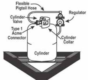
Single Cylinder
