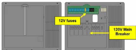
Typical Load Center Panel Load Center Panel w/120 volt Main Breaker
