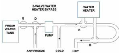
Two Valve Water Heater Bypass Valves shown in NORMAL mode
