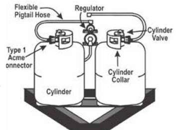
Double Cylinder
